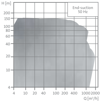
Performance curves
